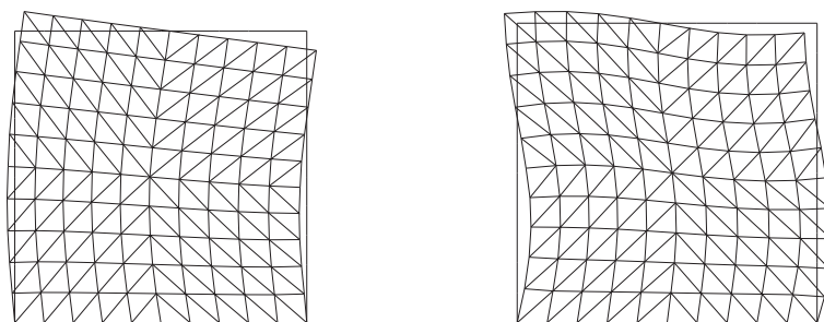
FIG. 6.3. Test 1 (AFW). Vibration modes associated with frequencies \omega_{h3} (left) and \omega_{h4} (right).
