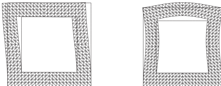
FIG. 6.5. Test 2 (PEERS). Vibration modes associated with frequencies \omega_{h1} (left) and \omega_{h2} (right).
