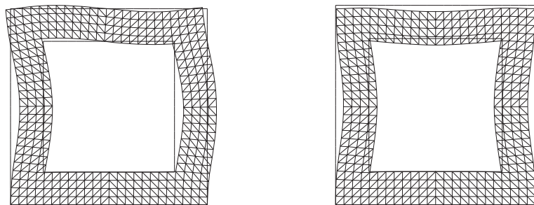
FIG. 6.6. Test 2 (PEERS). Vibration modes associated with frequencies \omega_{h3} (left) and \omega_{h4} (right).
