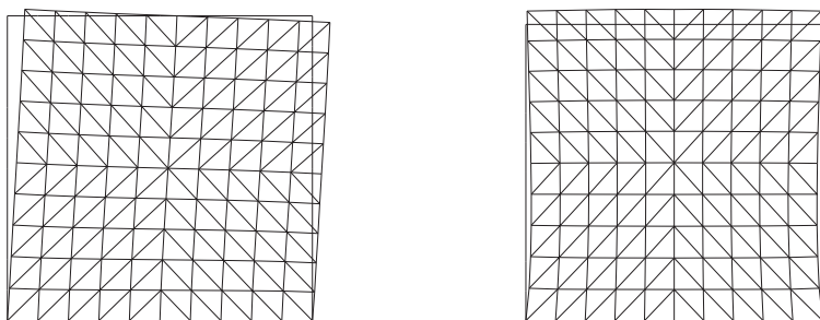
FIG. 6.2. Test 1 (AFW). Vibration modes associated with frequencies \omega_{h1} (left) and \omega_{h2} (right).
