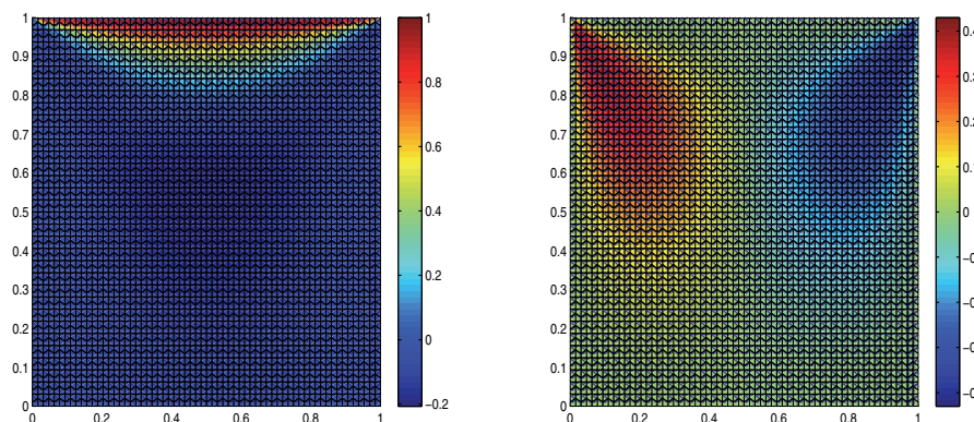
FIG. 5.4. The velocity profile and the stream function for the lid-driven cavity problem obtained with a triangular mesh (family \mathcal{T}_h^1 , h = 1/64 ).
